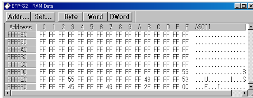
Fig. 6.2: Dump Window (ID Code Setting Data)
