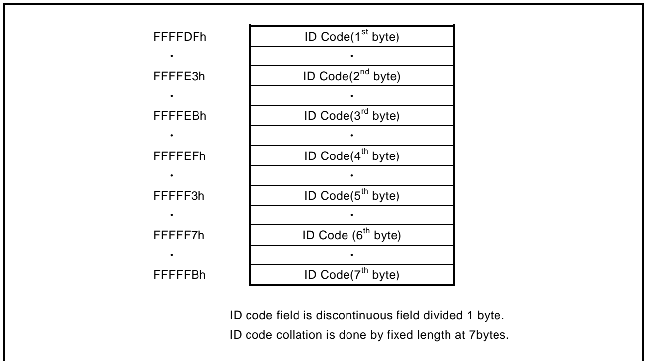
Fig. 5.1: ID Code Field Configuration
