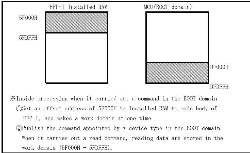
Fig. 6.2 Work domain diagrammatical view
