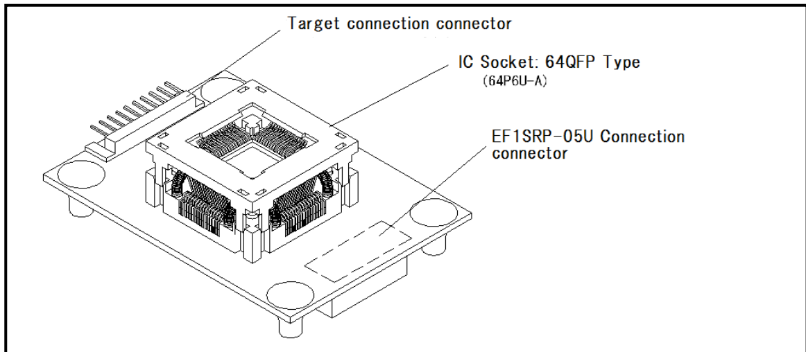
Fig.1.1 MS7282-64U External Figure
