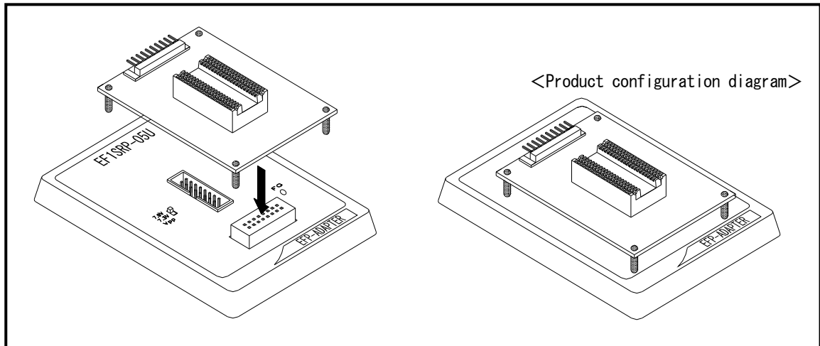
Fig 2.1 Connection with EF1SRP-05U
