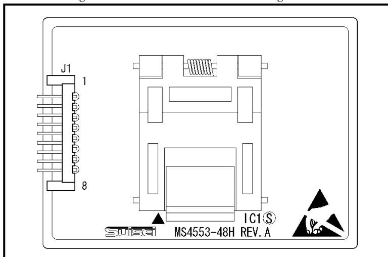
Fig 1.1 MS4553-48H External Figure
