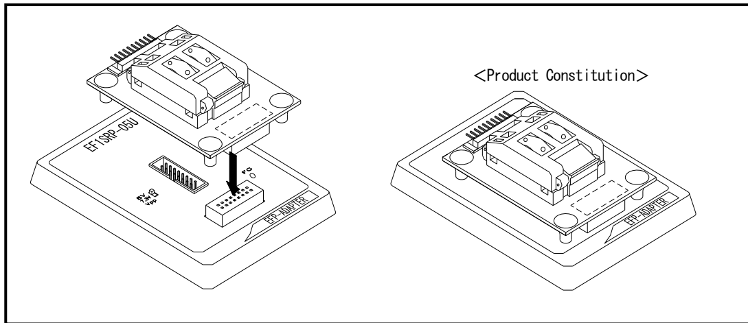
Fig. 2. 1 Connection to EF1SRP-05U
