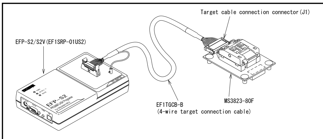
Fig. 2. 2 Connection to EF1SRP-01US2
