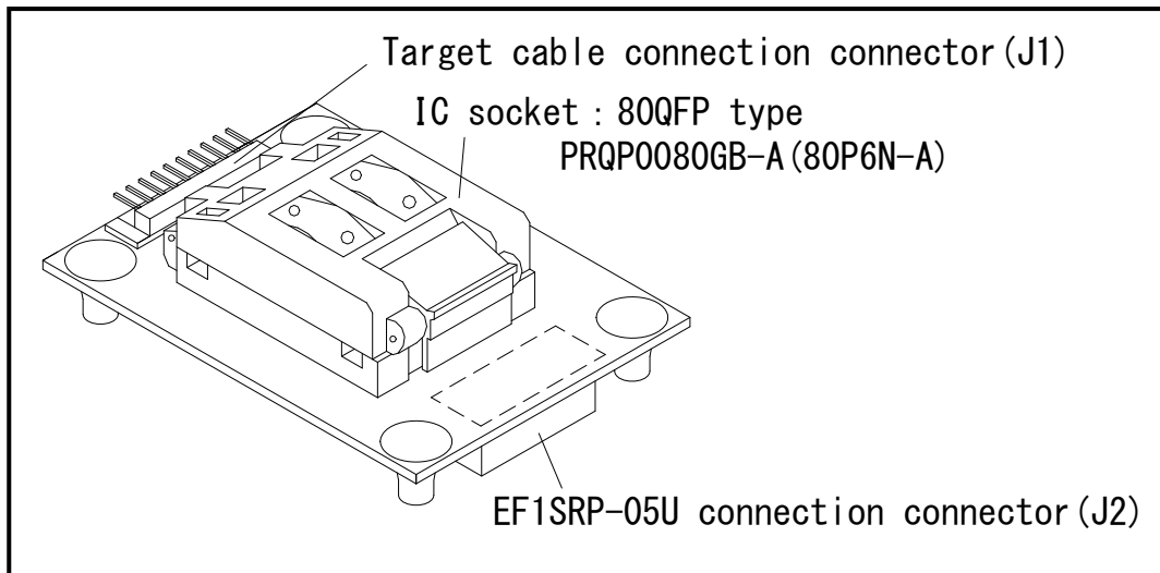
Fig 1.1 MS3823-80F External Figure
